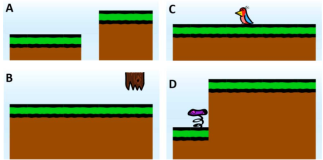
Fig. 2. Example instantiations of the four single-beat geometry patterns used in Tanagra. (A) A gap between two platforms. (B) A stomper. (C) An enemy. (D) A spring to a different platform. Patterns are described and produced using ABL behaviors. Note that there are many different configurations of each pattern; the precise placement of geometry is determined by the constraint solver (Choco).
