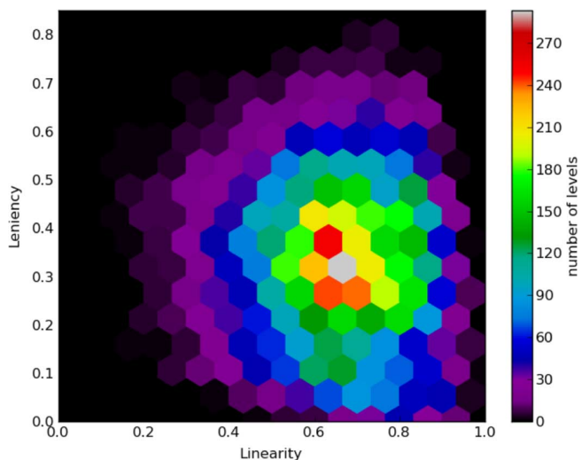
Fig. 11. Tanagra's expressive range, measured on the linearity and leniency of generated levels. 10 000 unique levels were generated and graded by these metrics. In this visualization, each hexagon corresponds to a bin containing levels and is colored by the size of each bin according to the scale on the right-hand side.
