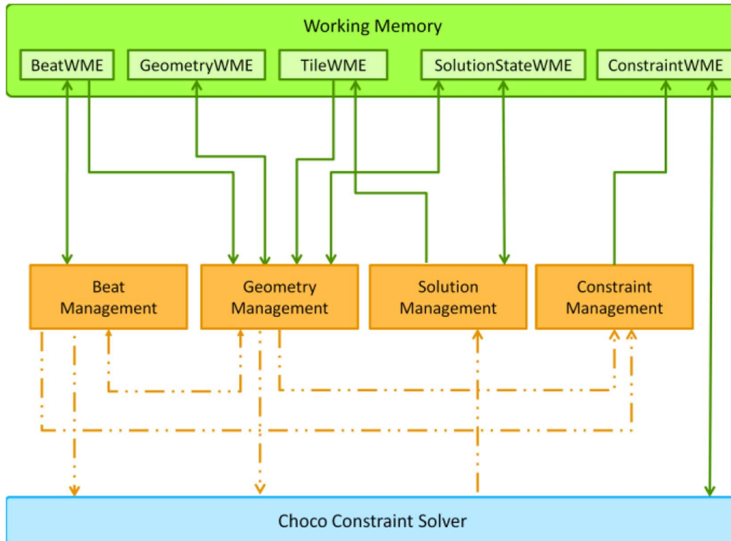
Fig. 6. This diagram shows the communication channels between working memory, ABL, and Choco, and dependencies between different managers within ABL. Green solid lines denote WME reading and writing, and orange dashed lines denote behavior and function calling.
