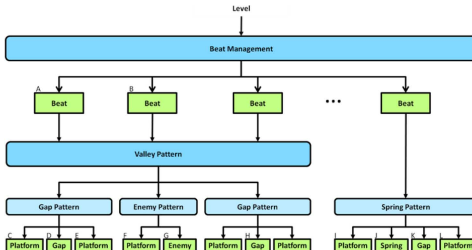
Fig. 7. A diagram representing a potential partial level during level generation. Blue, rounded boxes denote ABL behaviors. Green boxes are WMEs. Not represented here are the tiles that make up each level component. Table I provides examples of the constraints imposed between each level component.
