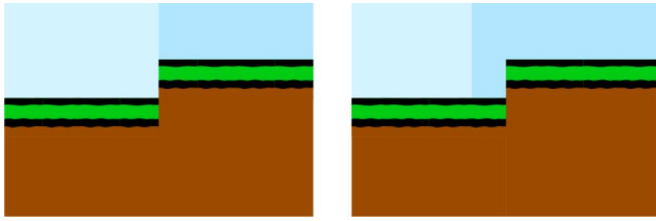
Fig. 8. The necessity for correcting beat placement based on geometry placement. The blue shaded boxes denote beat boundaries. If the designer draws geometry as depicted on the left-hand side, there can never be a solution to the level as the platforms do not line up at the beat boundary. However, this geometry placement should clearly be playable. The right-hand side shows how Tanagra corrects beat boundaries to address this issue.
