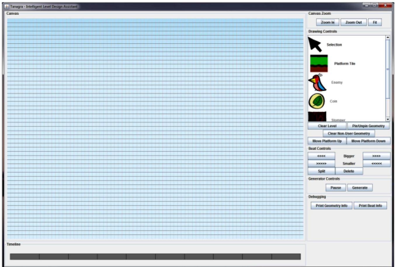
Fig. 3. The empty Tanagra editing environment. The blue gridded area in the upper left is the geometry canvas. Below that is the beat timeline. Along the right-hand side of the screen are the editing controls.
