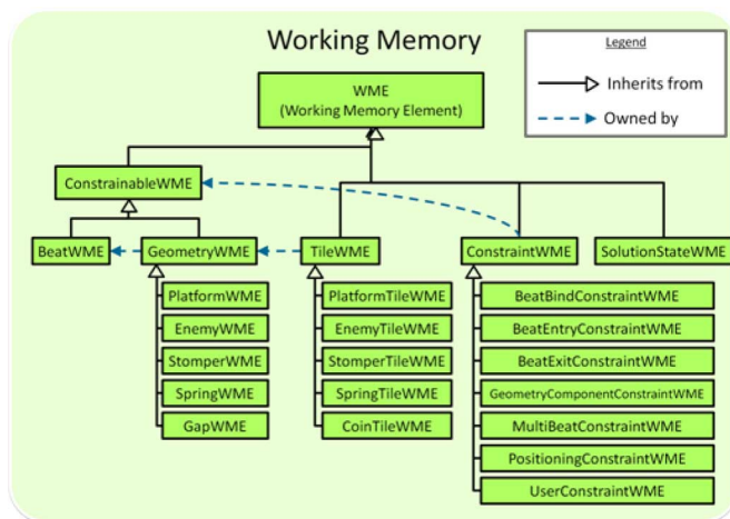
Fig. 5. The hierarchy of working memory elements used to represent levels in Tanagra. Solid, black arrows denote inheritance; dashed blue arrows denote ownership. For example, ConstraintWME s have multiple owners, each of which must be a ConstrainableWME .
