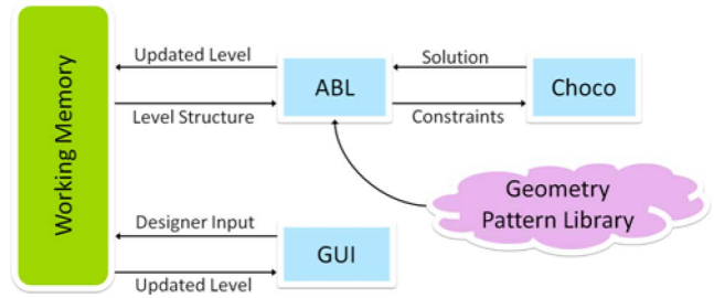
Fig. 4. Tanagra is made up of three main components: the GUI, an ABL agent, and the Choco constraint solver. The GUI and ABL communicate through working memory. ABL posts constraints to Choco and determines when the solver should be called; Choco responds with either a potential solution or a notification that no solution exists. A library of geometry patterns are specified using ABL behaviors.
